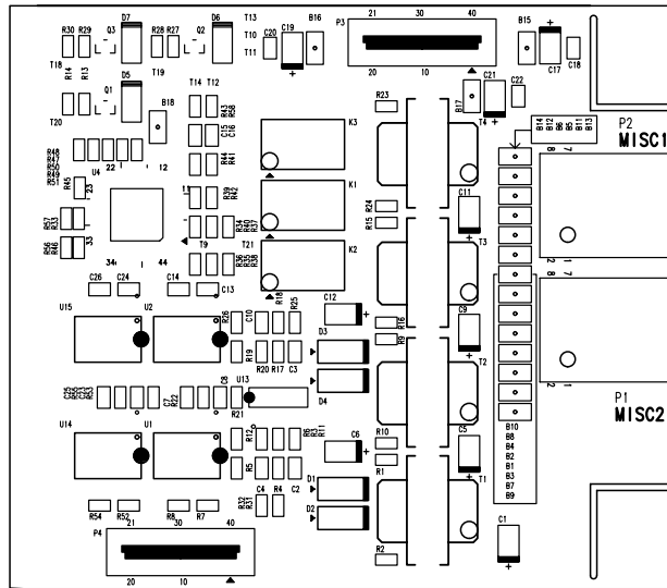
Figure 3-9 MISC Board
