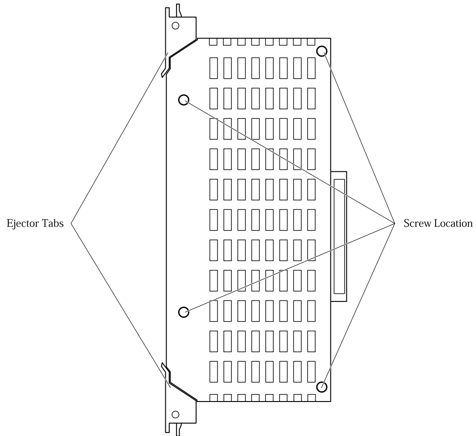
Figure 3-19 TEPR Card Screw Location
