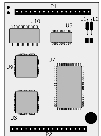
Figure 3-14 Modem Board
