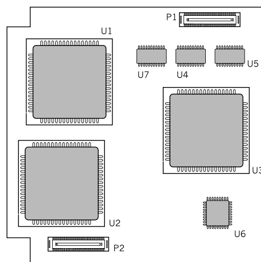
Figure 3-11 SCM Board
