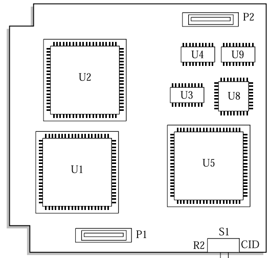
Figure 3-13 RCM Board
