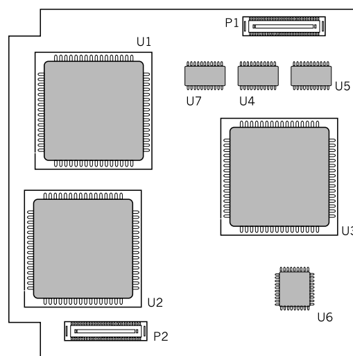
Figure 3-12 MFM Board
