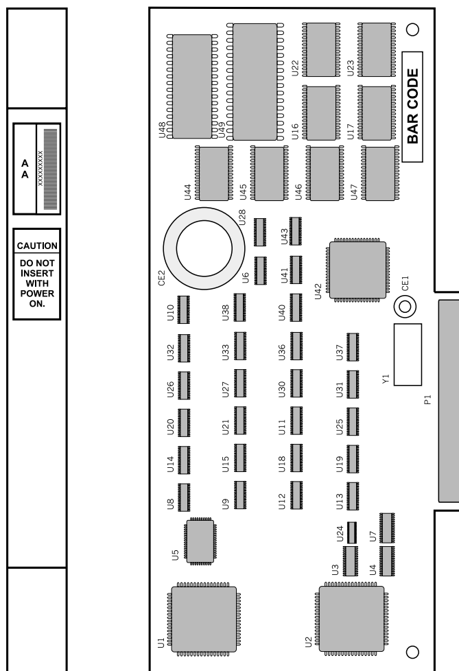
Figure 3-20 AAUCD Card
