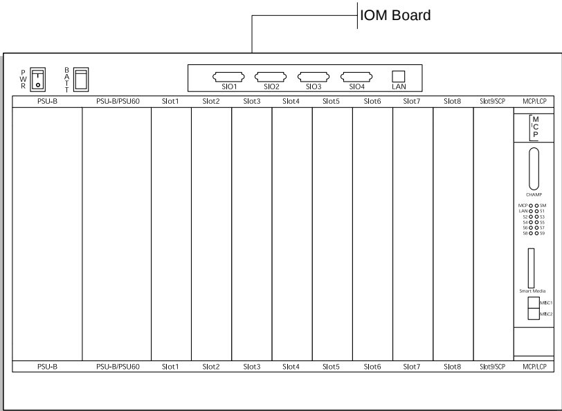
Figure 3-16 Cabinet/Slot Numbers
