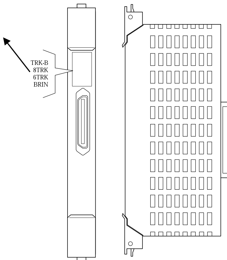
Figure 3-17A Interface Cards
