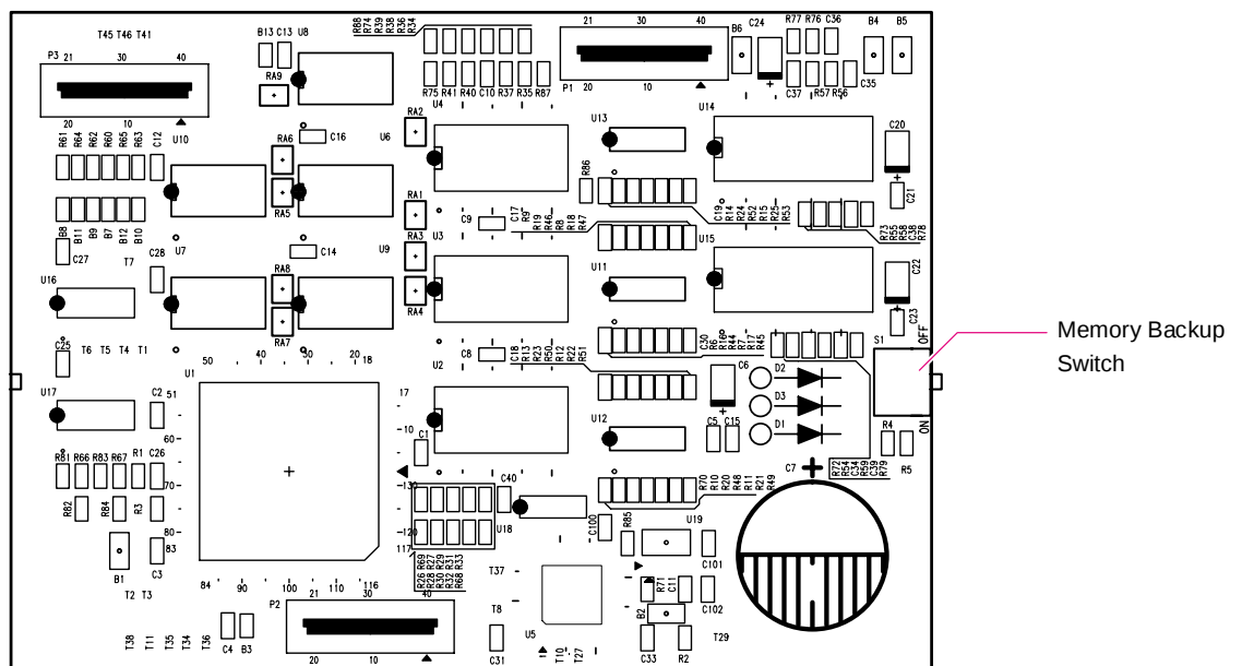
Figure 3-7 IPM Board
