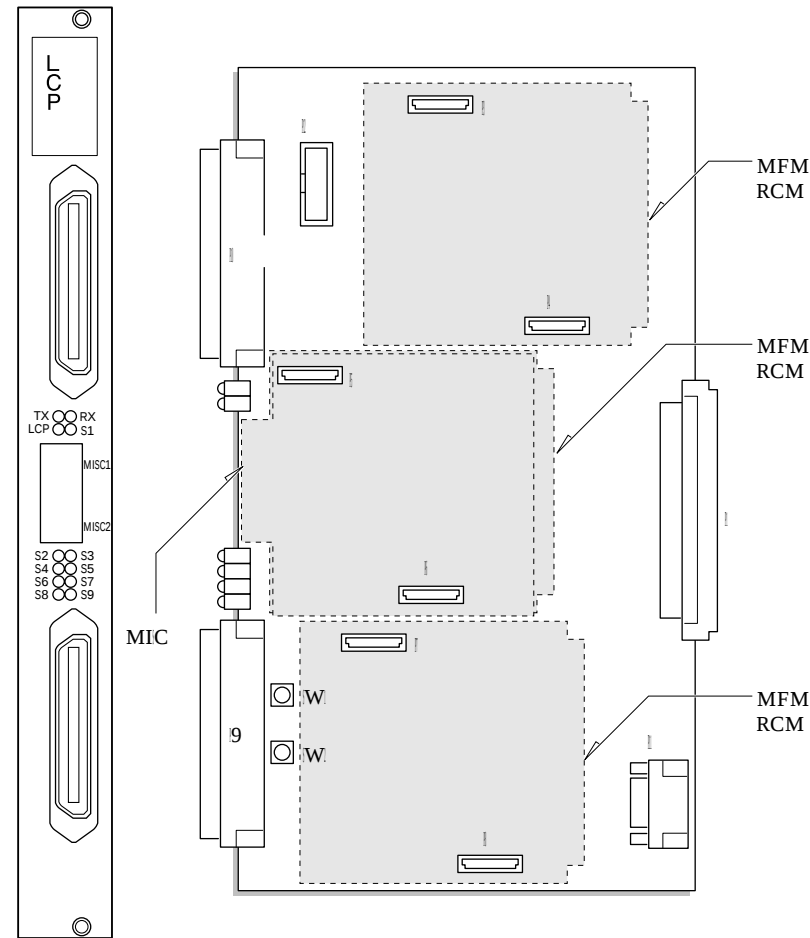
Figure 3-4 LCP Card
