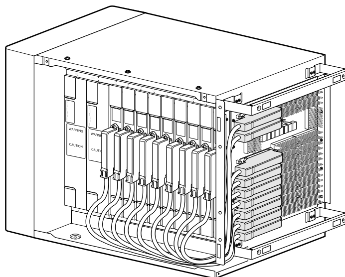
Figure 2-10 Connecting Champ Cables to the MDF boards
