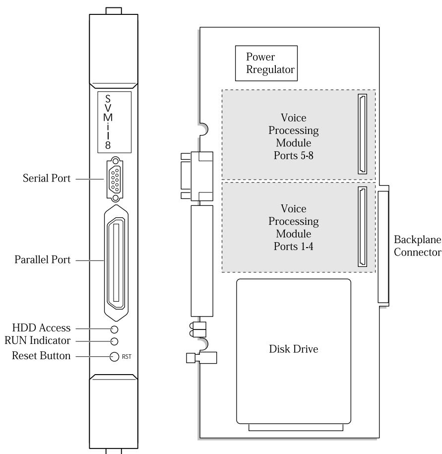
Figure 3-21 SVMi-8 Card
