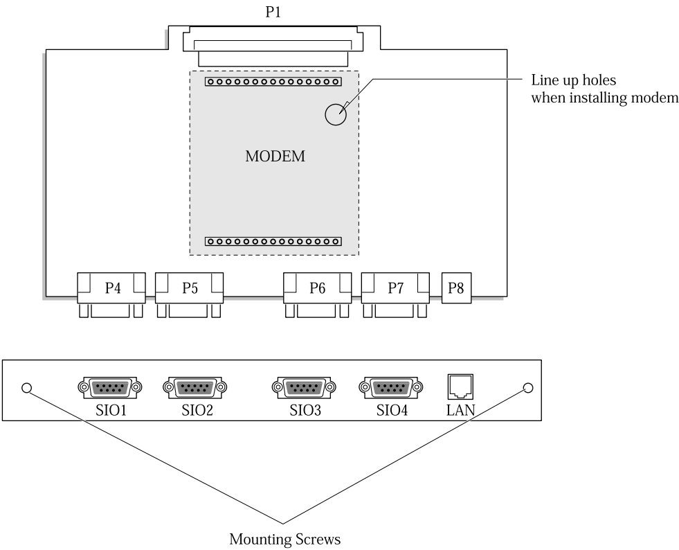
Figure 3-15 IOM Board
